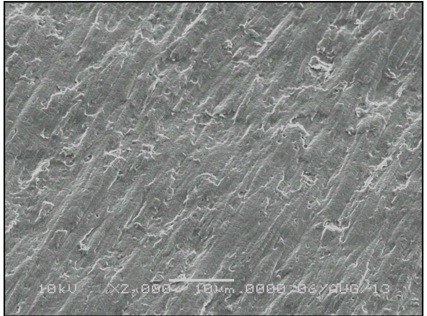
Matt side of raw copper foil (elettroscanningmicroscope2000x)
